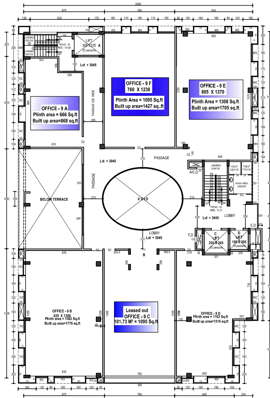
9th FLOOR PLAN
