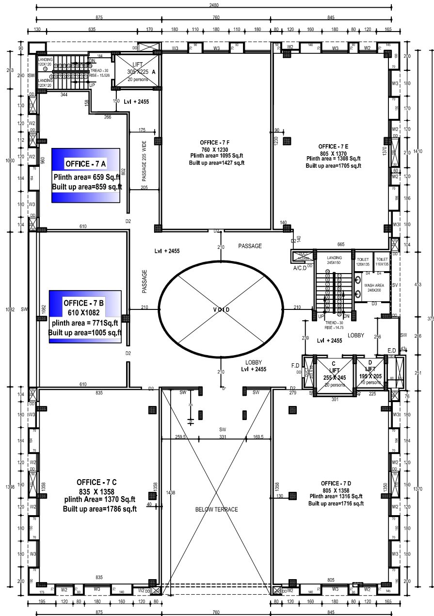
7th FLOOR PLAN
